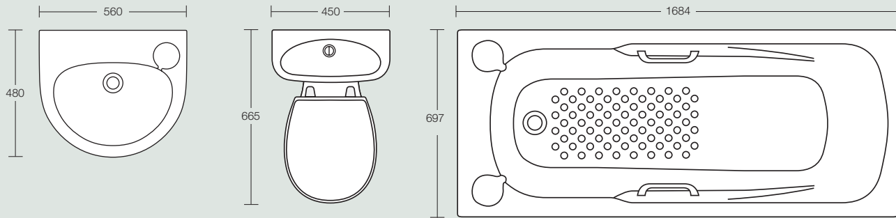
Sandringham 560mm pedestal washbasin Height 815mm 1 or 2 tapholes (full pedestal mounted)
