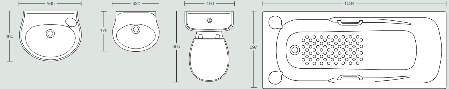
Sandringham Classic 560mm pedestal washbasin Height 855mm 1 or 2 tapholes (full pedestal mounted)
